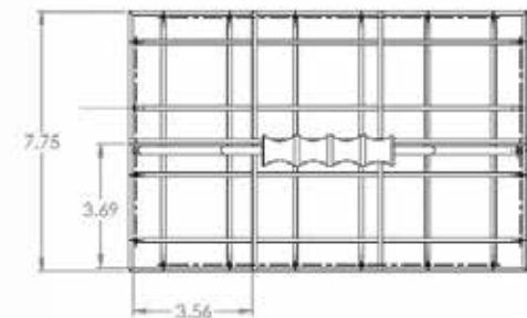
6 CELL QUART CARRIER
