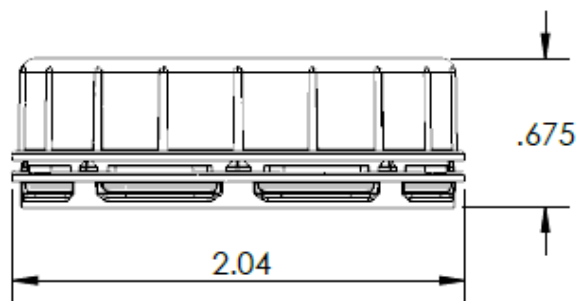
48 MM NECK FINISH
