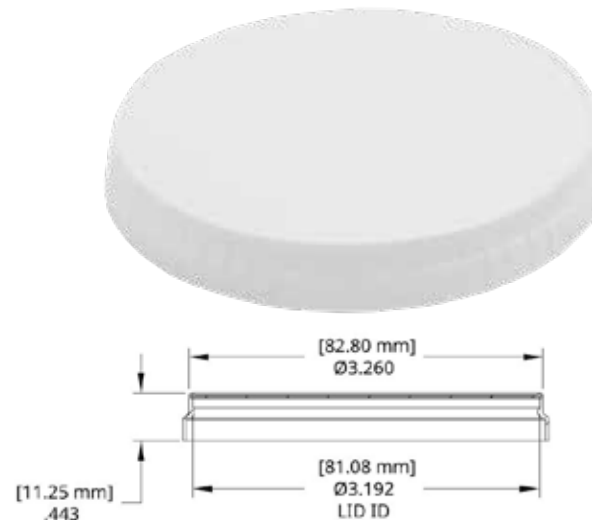
82 MM PAPER LID
