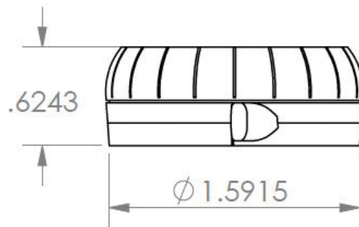
38 MM NECK FINISH
