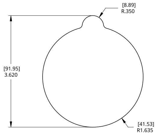
83 MM (3.27") HEAT SEAL
